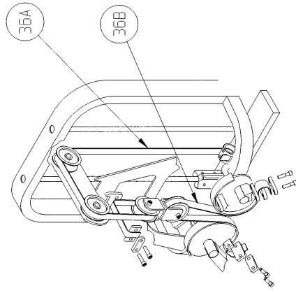
BELT ROUTING DETAIL
