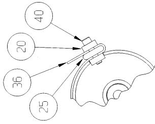
BELT CLAMPING DETAIL
